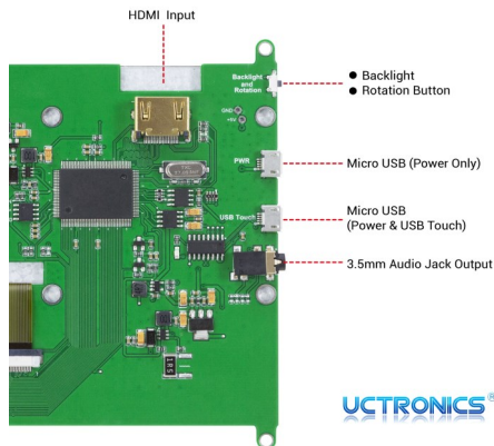
The connectors on the back of the display
